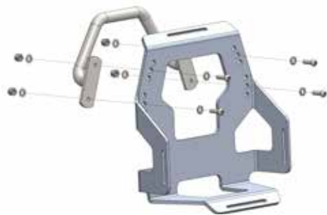
Mounting on C-Bow basic holder
