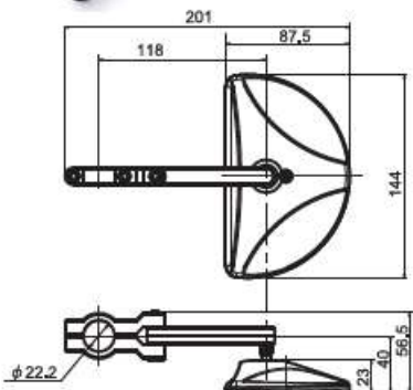
#81001 Handlebar clamp type 1PC
