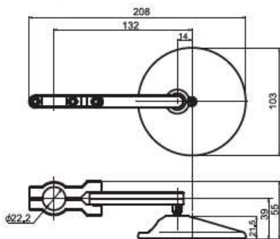
#80917 Handlebar clamp type 1PC
